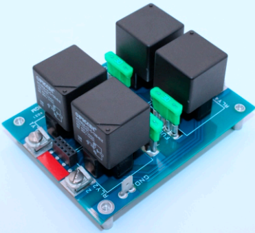
Replacement relay board for 4000 Series Control Modules
