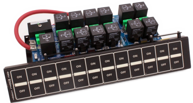
12001RP Flat Touch with Oil Pressure Control
