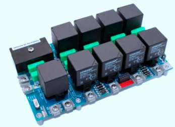
Replacement relay board for 8000 Oil Pressure Control Modules Series Control Modules
