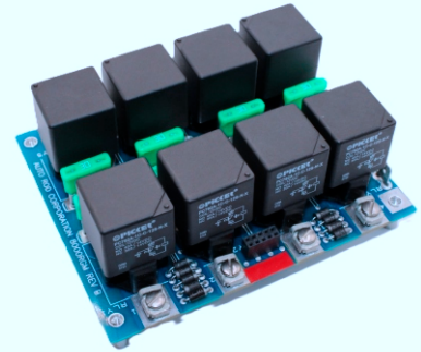
Replacement relay board for 8000 Series Control Modules
