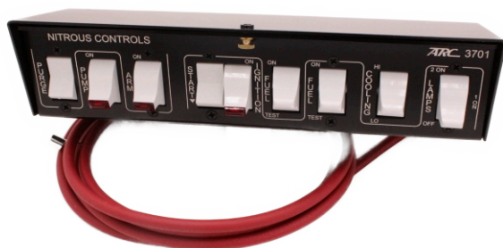
11-3/8" L x 2-5/8" H x 3-1/2" D
