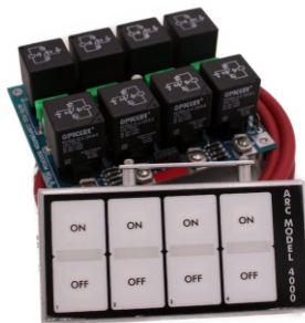
4-7/8" L x 2-3/8" H x 3/4" D
