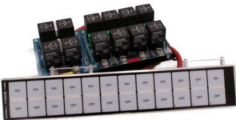
13" L x 2-3/8" H x 3/4" D
